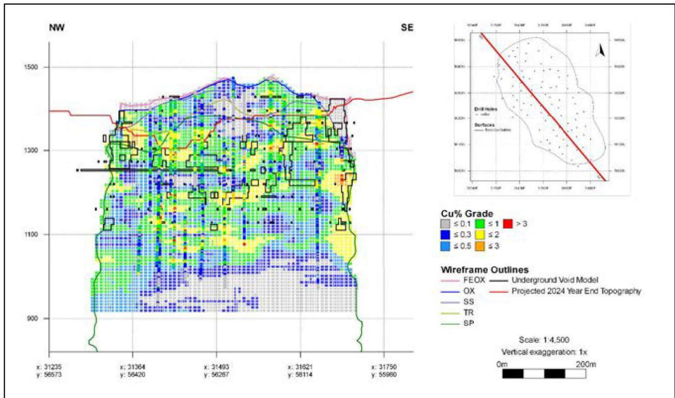
Figure 11.39: NW-SE Cross-section of Composite Samples and Block Grades ± 20 m
