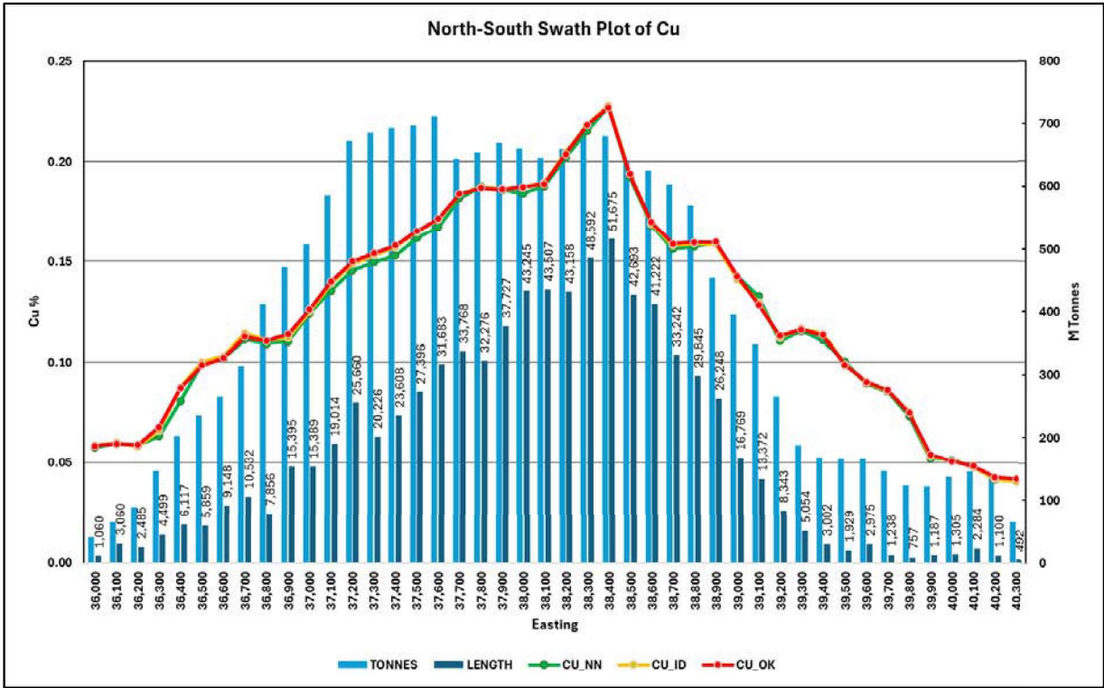
Figure 11.18: North-South Swath Plot of Cu %
