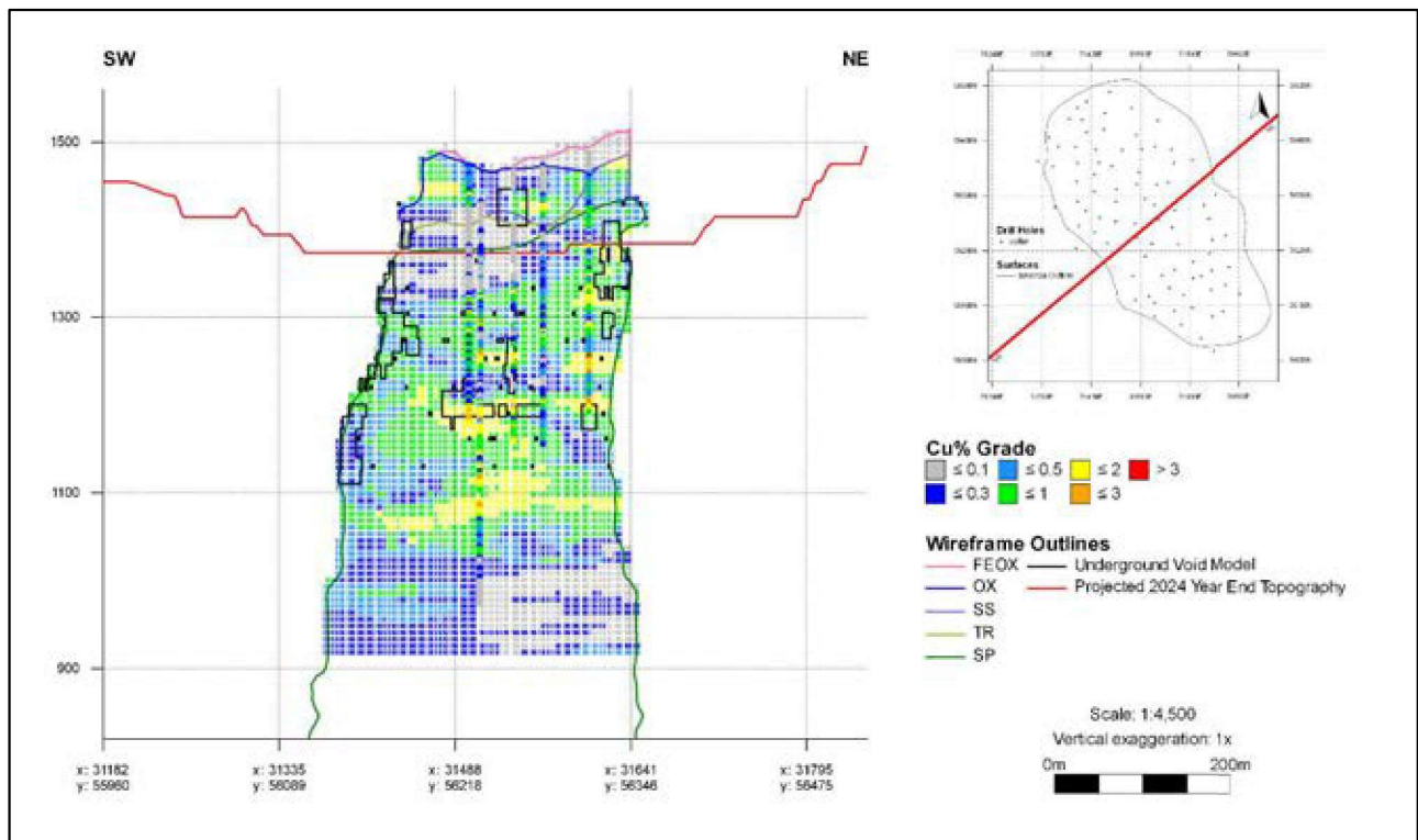
Figure 11.40: SW-NE Cross-section of Composite Samples and Block Grades ± 20 m
