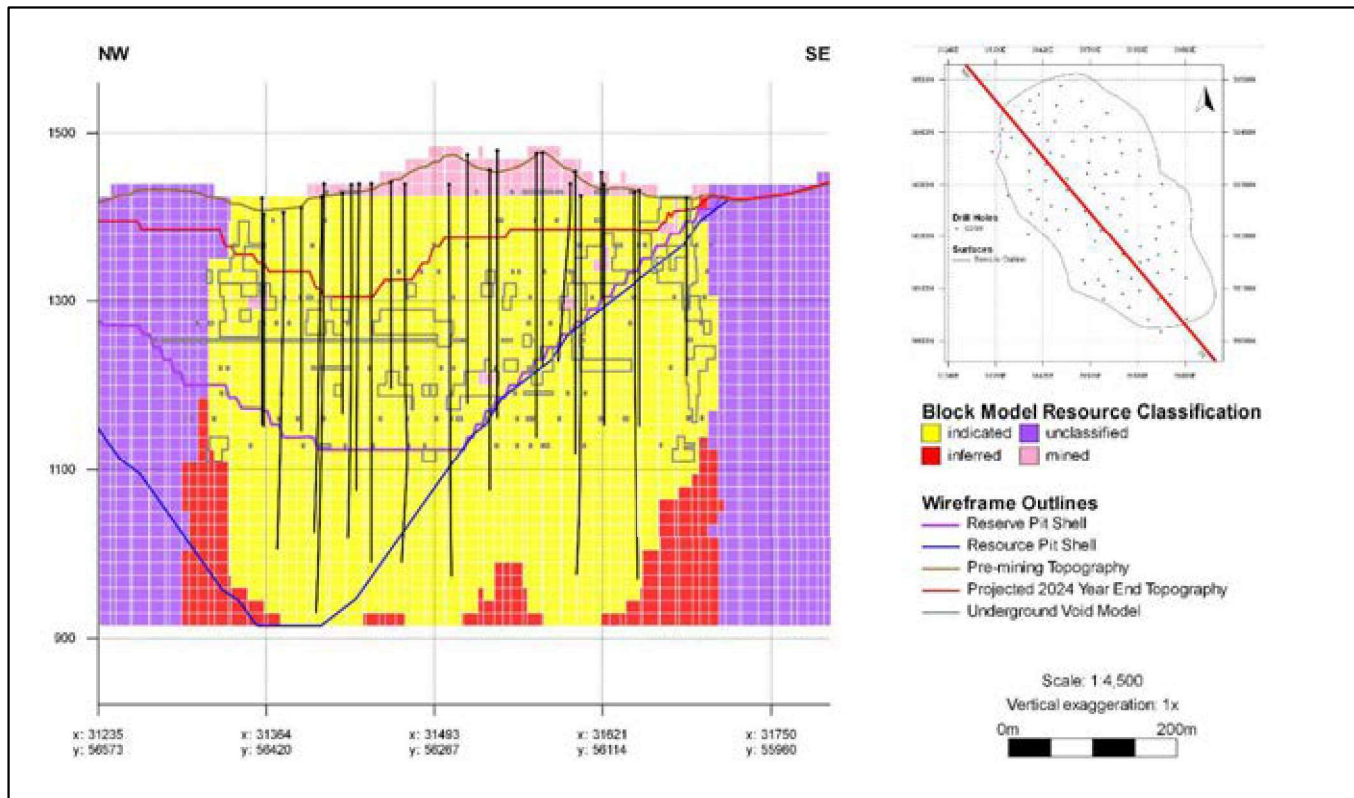
Figure 11.50: Pilares NW-SE Cross-Section Resource Classification Assigned to the Block Model
