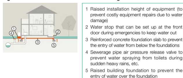
Figure 2. Measures to Prevent Underfloor Flooding
