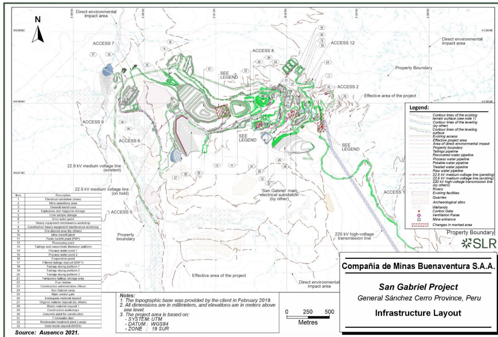
Figure 15-1: Site Infrastructure
