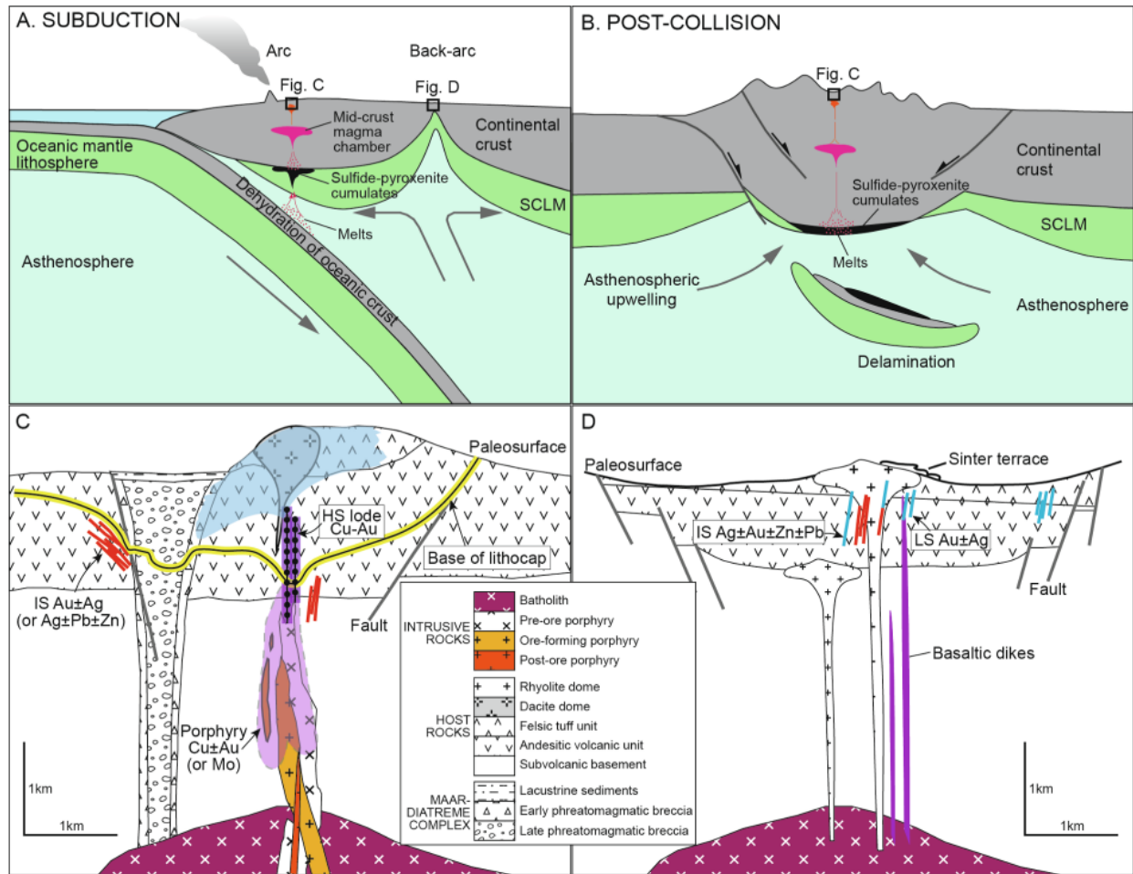
Figure 6-13: Classification of Intermediate Sulphidation Epithermal Deposits
