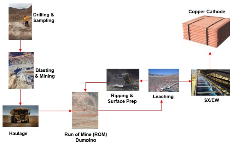
Figure 14.3 – Hydrometallurgical Process Diagram
