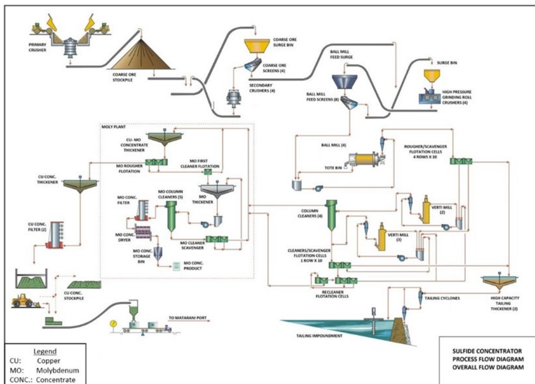
Figure 14.4 – Mill Process Diagram
