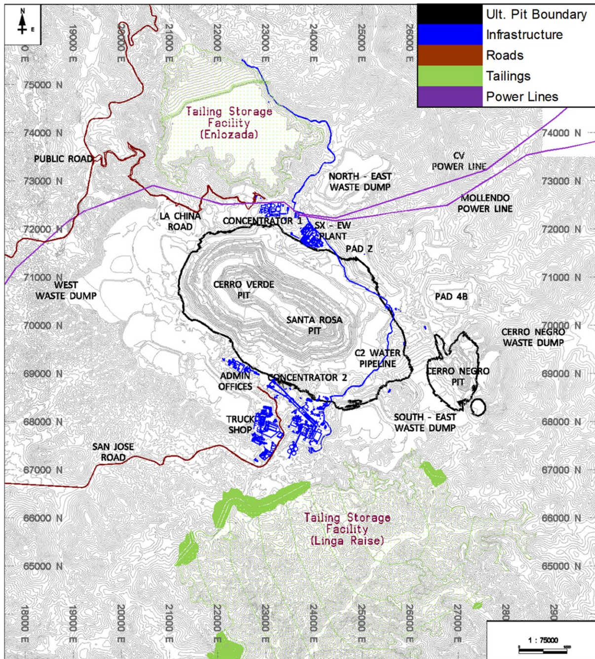
Figure 15.1 – Site Infrastructure Map
