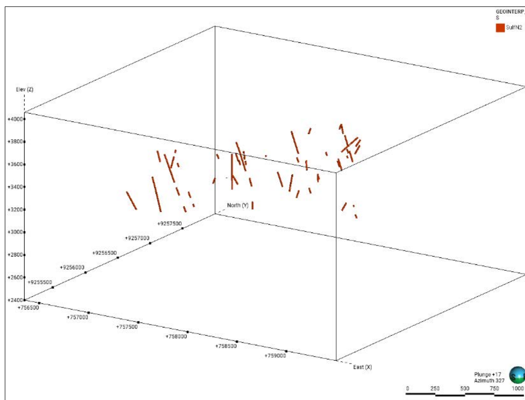
Figure 11-36: Sample support corresponding to the “SulfN2 / Epithermal Porphyry” domain in the “GEOINTERP_1S” column.
