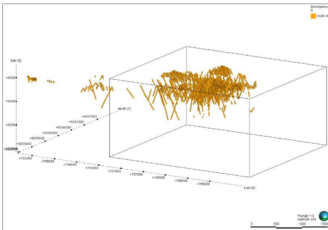
Figure 11-19: Sample support corresponding to the domain “ArglAvd2” in the “Description_1S” column.
