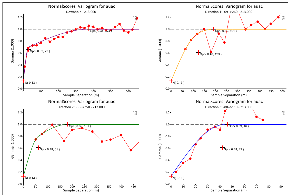
Figure 11-52: Modeled variogram for Au in the domain 213.
