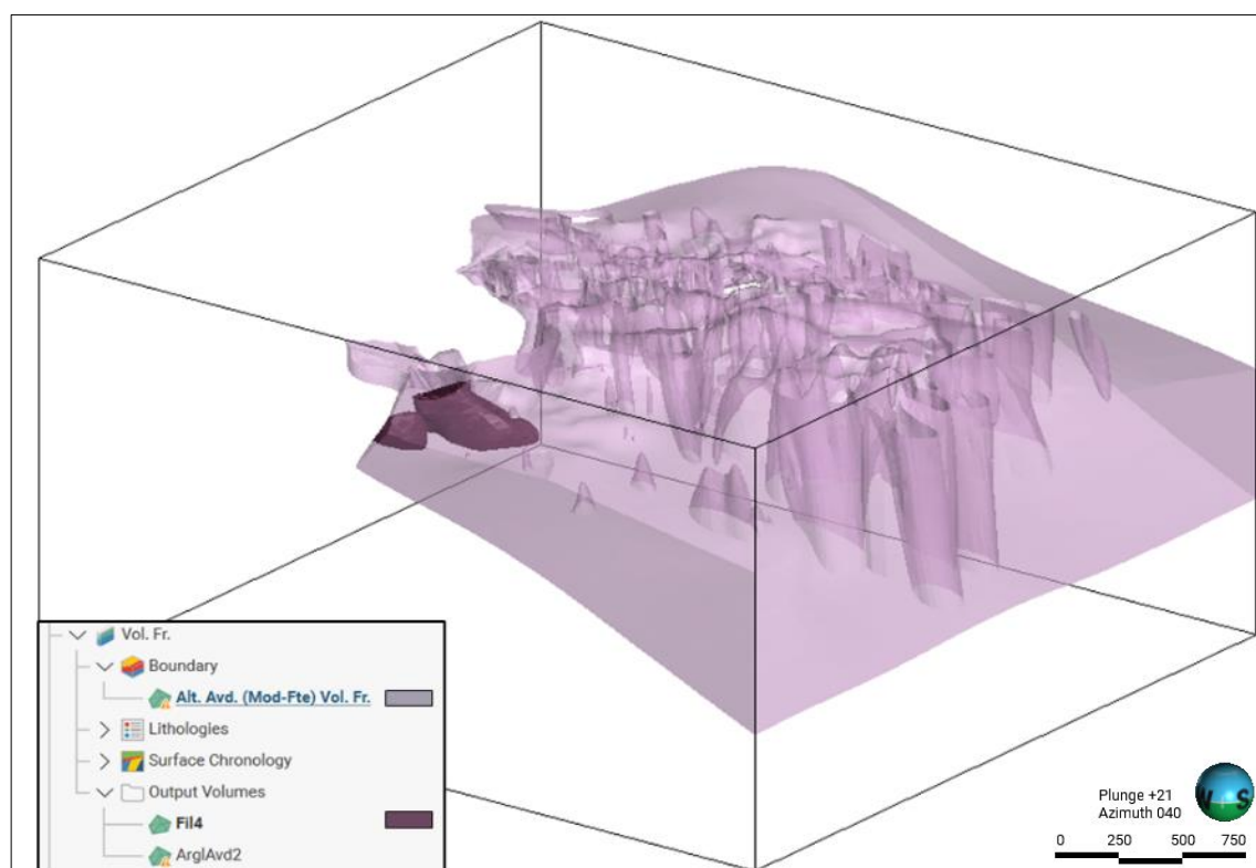
Figure 11-3: Wireframe of the “Phyllic” domain of the alteration model.
