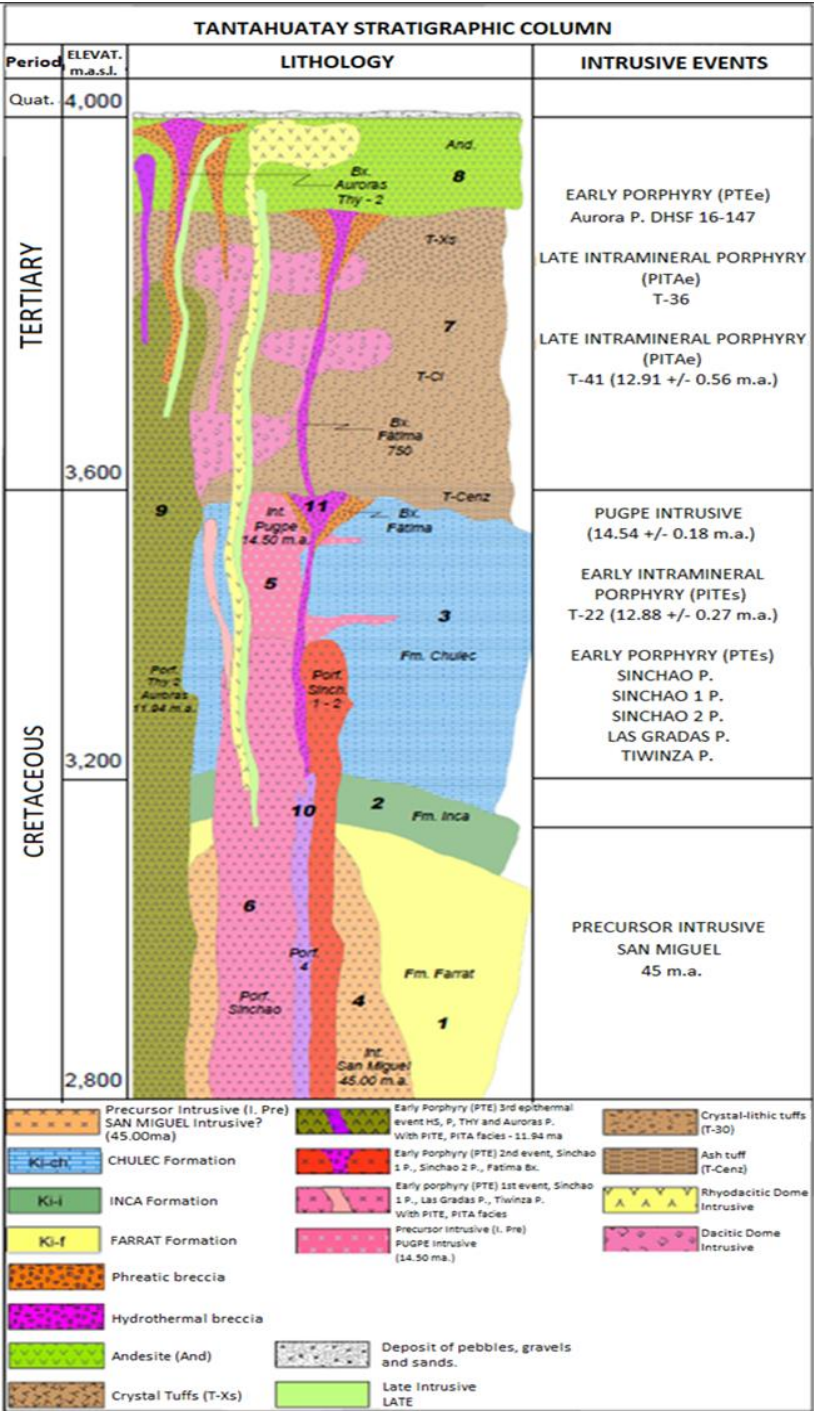
Figure 6-3: Stratigraphic column of Tantahuatay volcanic complex.
