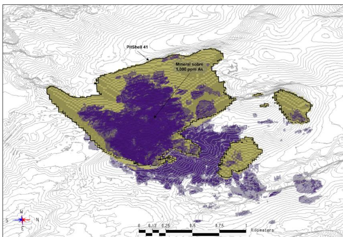
Figure 11-73: 3D View of ROM mineral over 1,000 ppm As.
