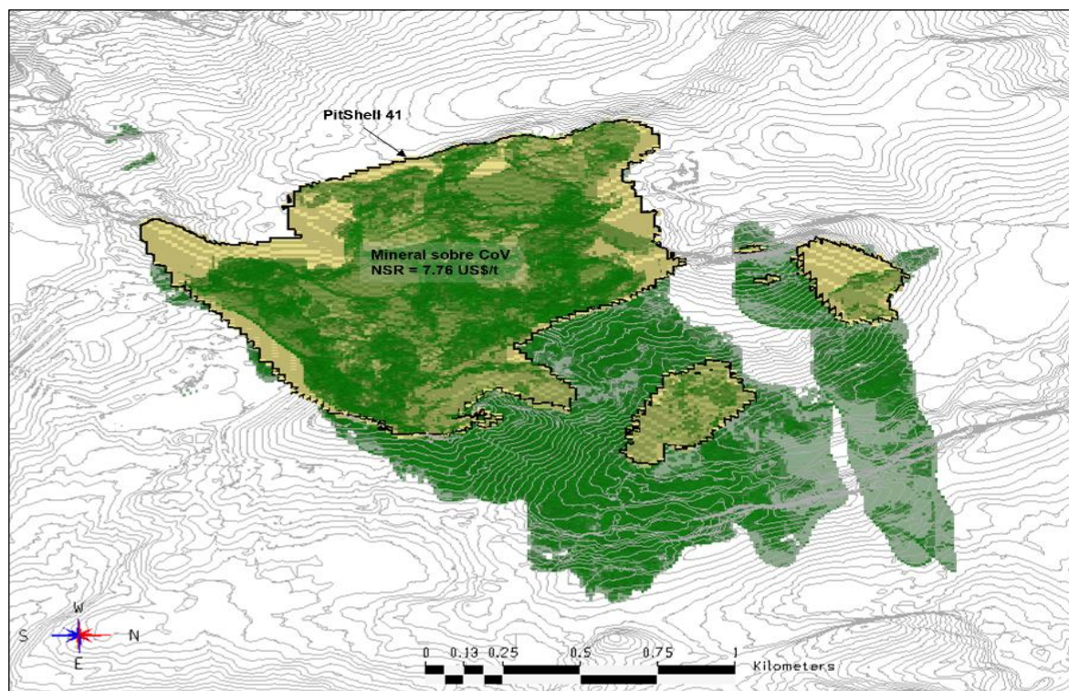
Figure 11-71: 3D View Mineral Resources economic cone
