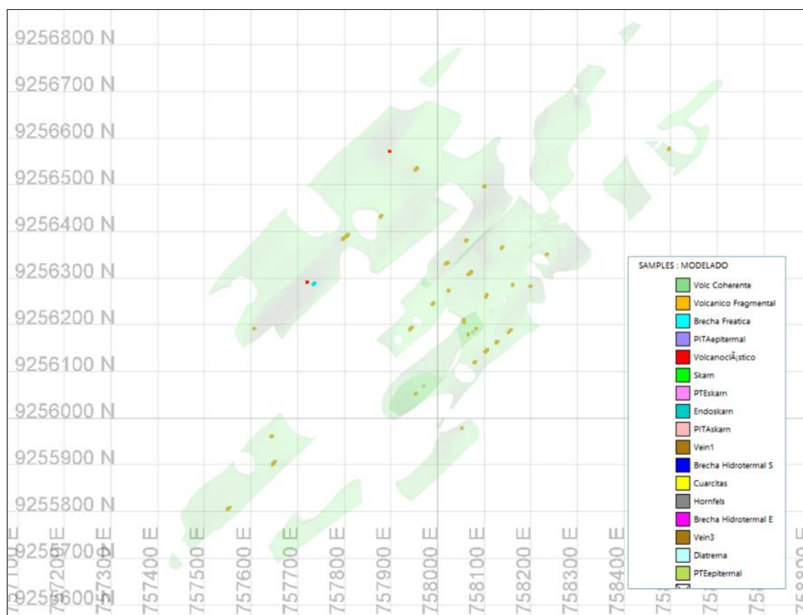
Figure 11-4: Plan view of the Vein1 domain, with the display of the samples found inside.
