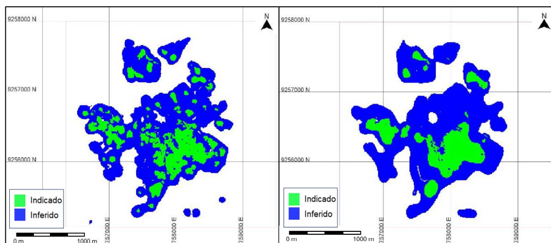
Figure 11-67: Plan view of the Tantahuatay Sulfuros mineral resource model, before and after smoothing.
