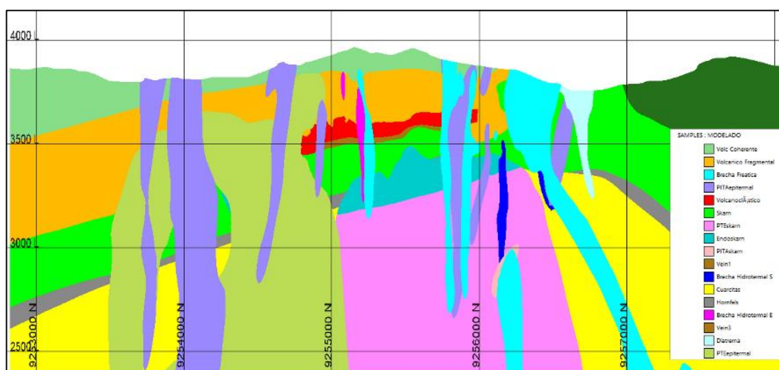
Figure 11-17: SW-NE Central Section of the Tantauhuatay Lithology Model.
