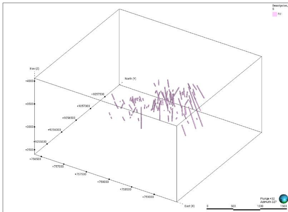
Figure 11-23: Sample support corresponding to the “Fil1” domain in the “Description_IS” column.
