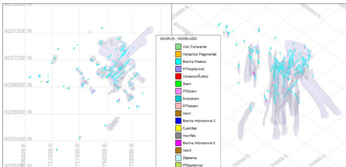
Figure 11-10: Phreatic Breccia domain with the distribution of the samples found inside with.
