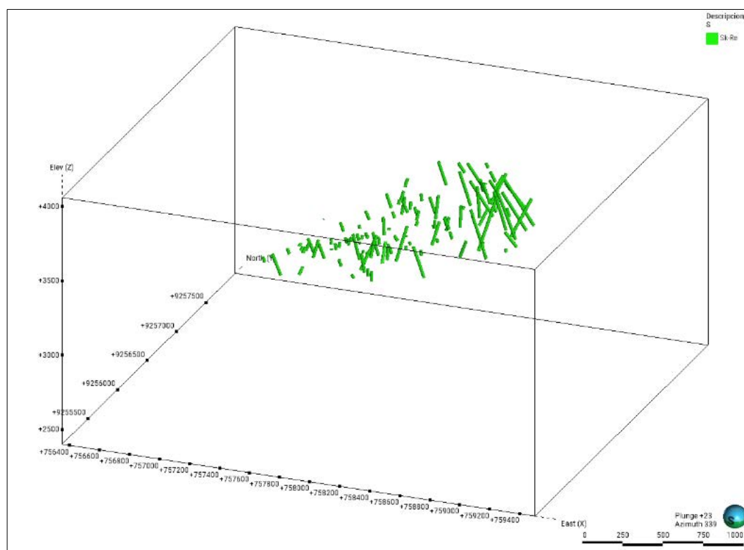
Figure 11-27: Sample support corresponding to the “Sk-Re” domain in the “Description_IS” column.
