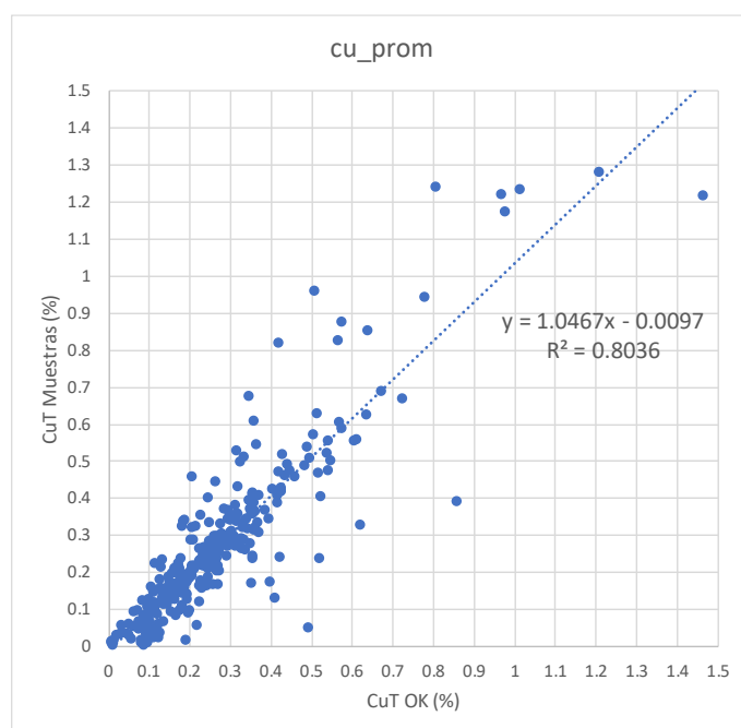
Figure 11-53: Conditional Bias review for domain 183.
