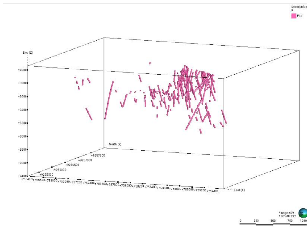
Figure 11-21: Sample support corresponding to the “Fil2” domain in the “Description_IS” column.
