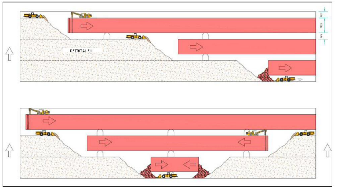
Figure 13-4: B&F mining diagram
