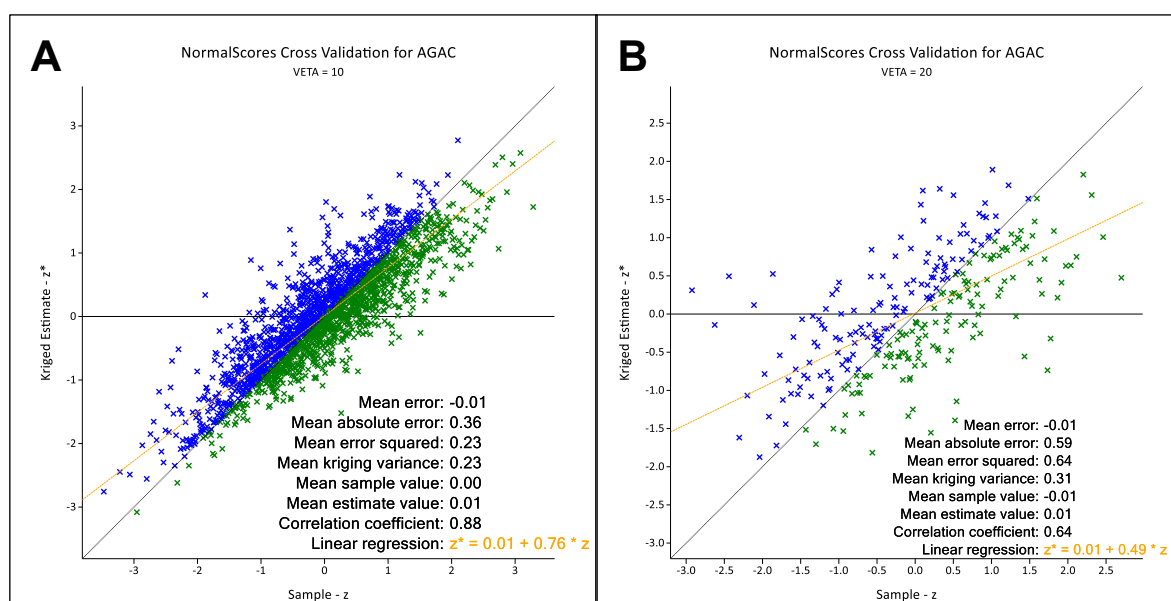
Figure 11-36: Cross Validation for Camila structure in domain 10 (A) and 20 (B) for Ag
