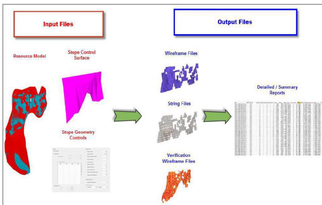
Figure 11-45: Input and output files after RPEEE analysis
