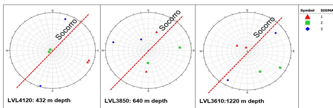
Figure 13-16: Orientation of in situ stresses measured at Uchucchacua
