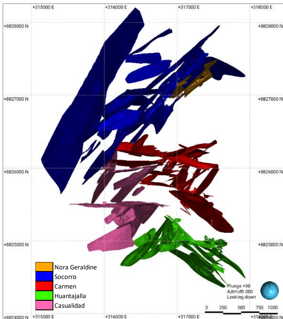
Figure 11-3: Modeled structures in the Uchucchacua Mine
