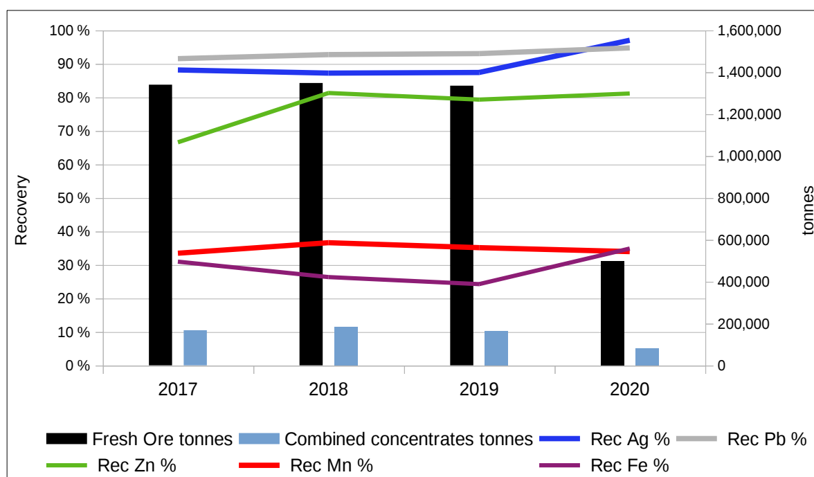
Figure 10-2: Uchucchacua Annual Process Plant Performance
