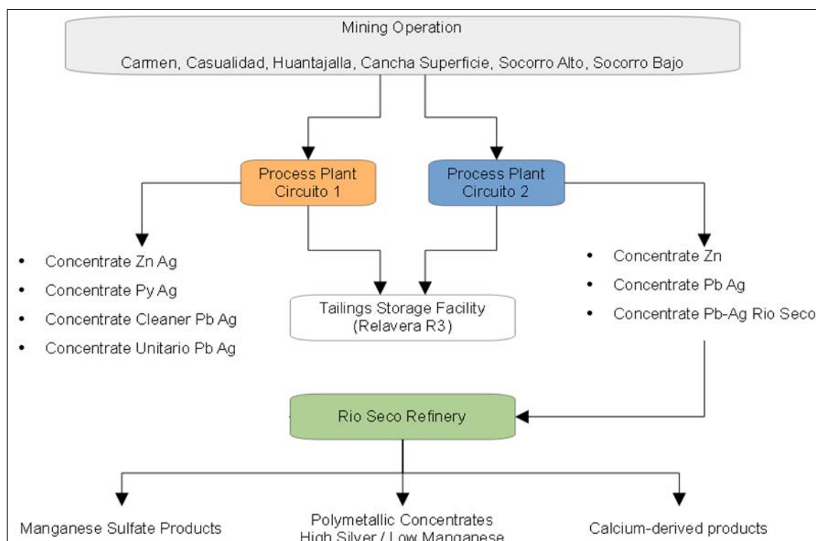
Figure 10-1: Uchucchacua, Simplified Block Flow Diagram
