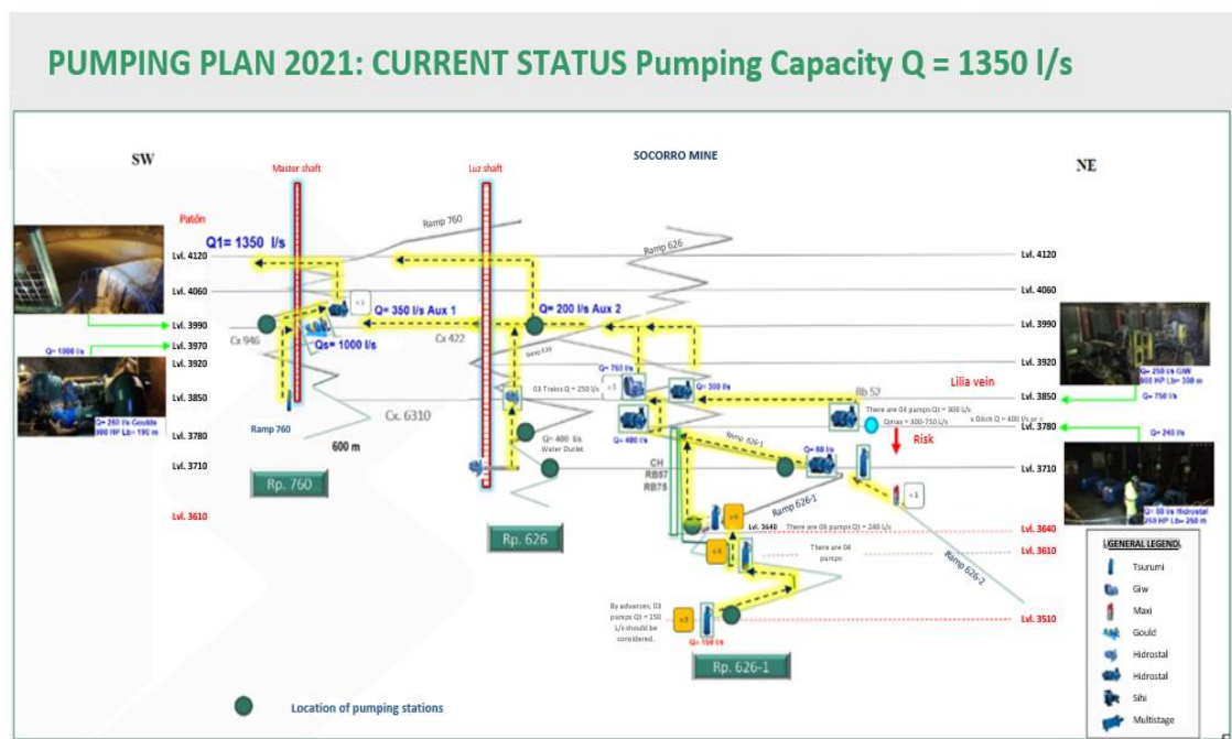
Figure 13-22: Current pumping system of Uchucchacua A.E.U.
