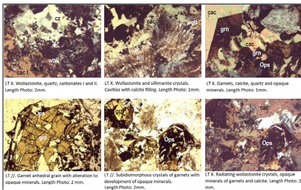
Figure 6-10: Thin sections of mineralization at Uchucchacua
