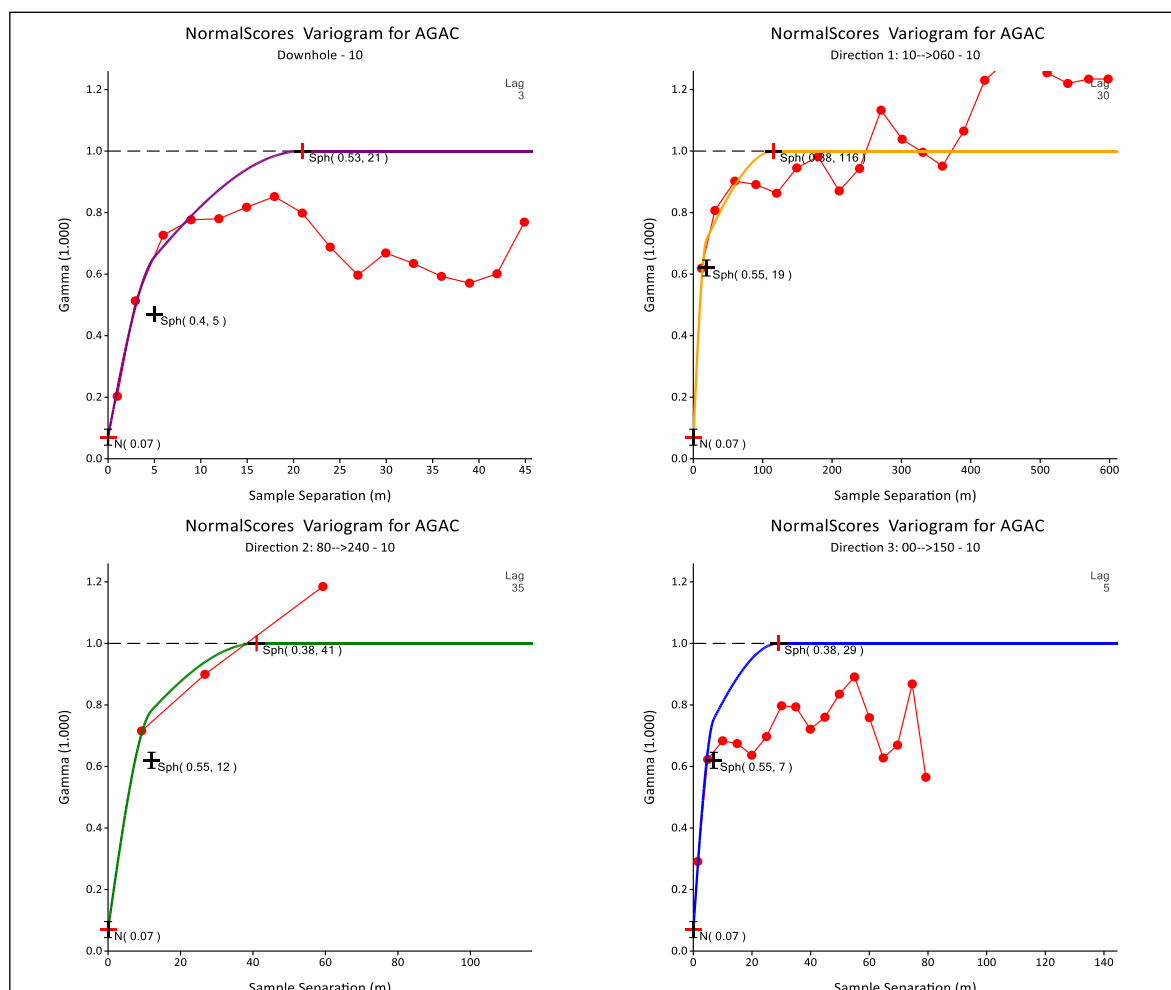
Figure 11-31: Variography of Camila Structure's domain 10
