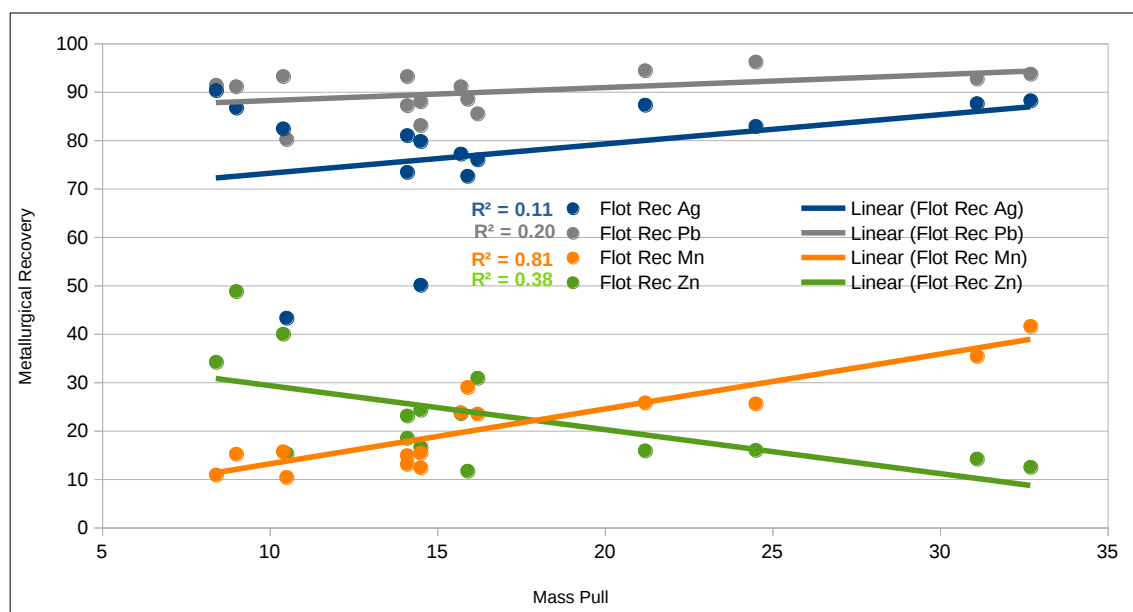
Figure 10-14: Yumpag, Recovery v/s Ore Mass Pull
