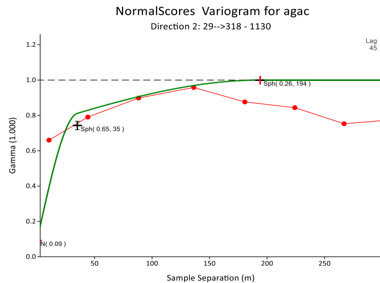
Figure 11-11: Variography of Gina Vein (1130)
