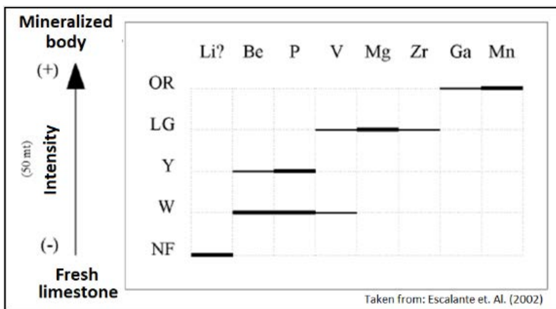
Figure 6-12: Calcite fluorescence.
