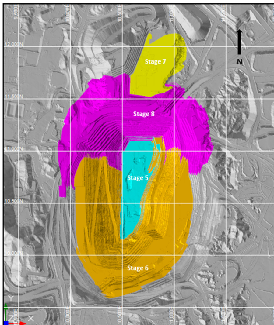
Figure 13.1. Remaining open pit stages at Sukari open pit.
